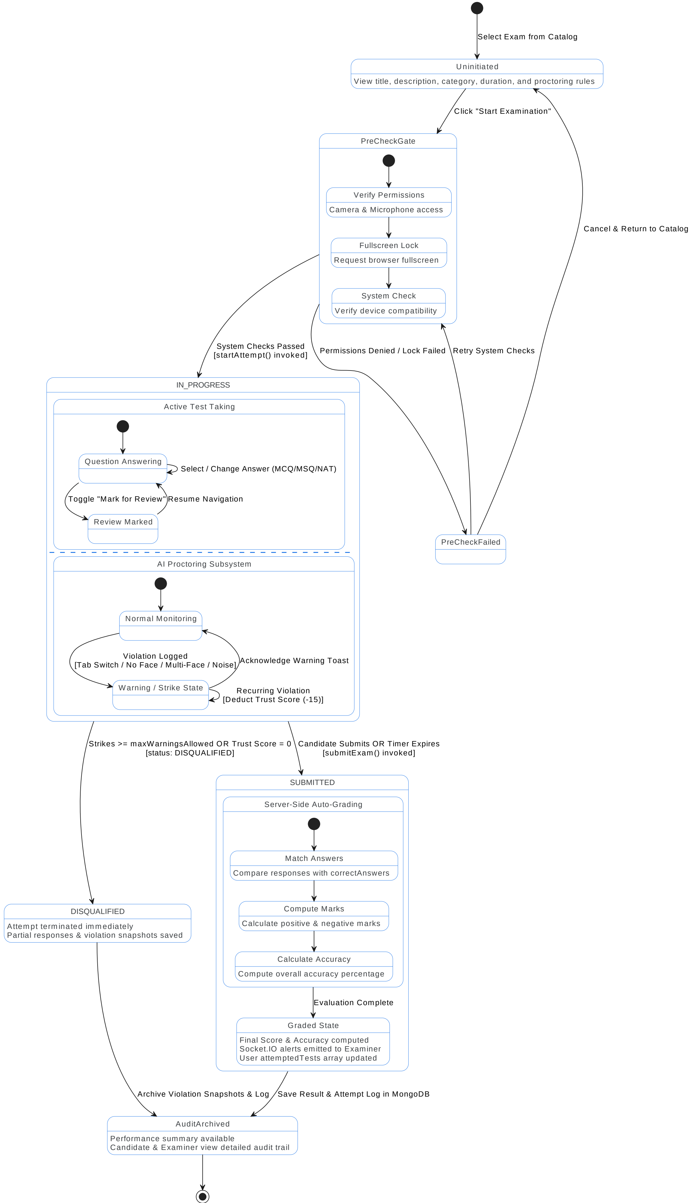
Mock Test Canvas State Machine Diagram
